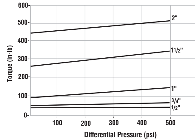
Polyfill Seats 1/2" - 2" Series WK70 Clean Valves
